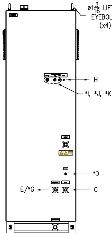
BACK VIEW
