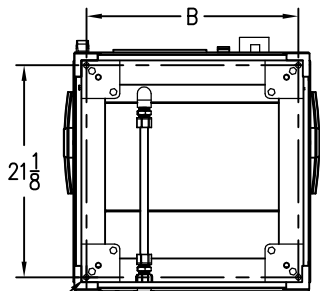
BOTTOM VIEW MOUNTING HOLE LOCATIONS
