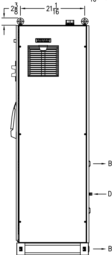
RIGHT VIEW
