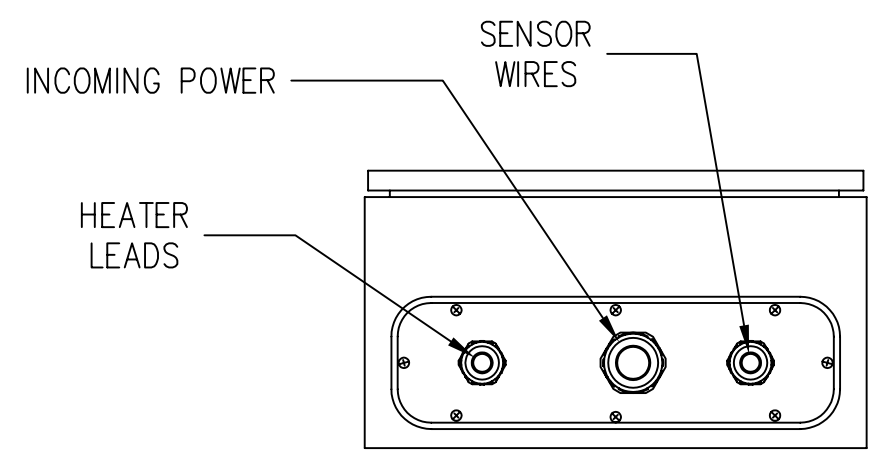
ELECTRICAL CONTROL CABINET
